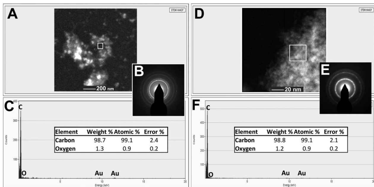
Figure 7. Scanning transmission electron microscopy (STEM) images (A, D), selected-area electron diffraction patterns (B, E), and energy-dispersive X-ray spectrometry plots (C, F) for elemental abundance of carbon: Younger Dryas Boundary nanodiamonds (NDs) from Lake Cuitzeo (493 ppb at 280 cm below surface; A–C) and synthetic NDs from PlasmaChem (D–F). Carbon in both is greater than \approx 98\% . HAADF = high-angle annular dark field. A color version of this figure is available online.
